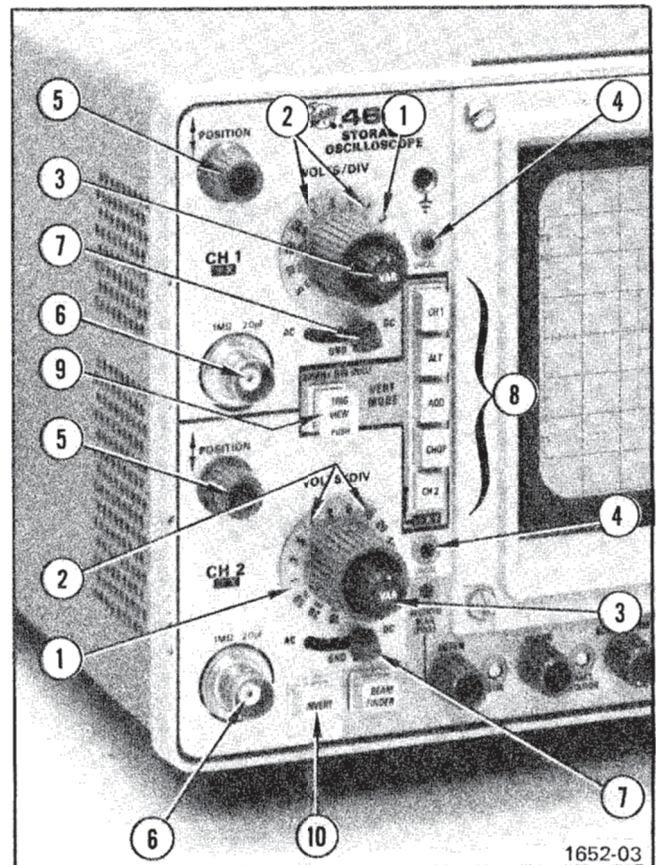
Fig. 2-2. Vertical Section.
