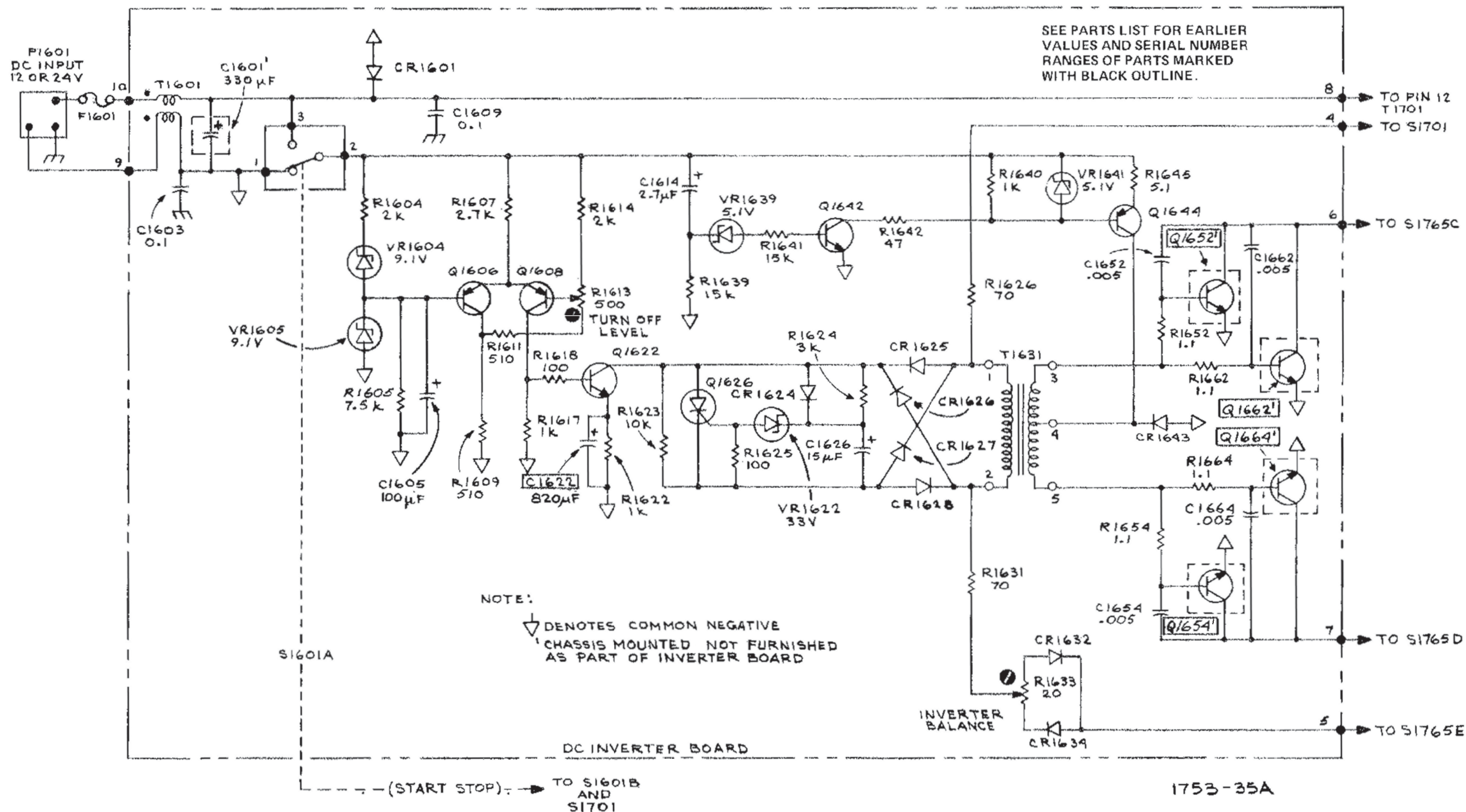
Figure Option 7-5. 466 Option 7 dc inverter.
