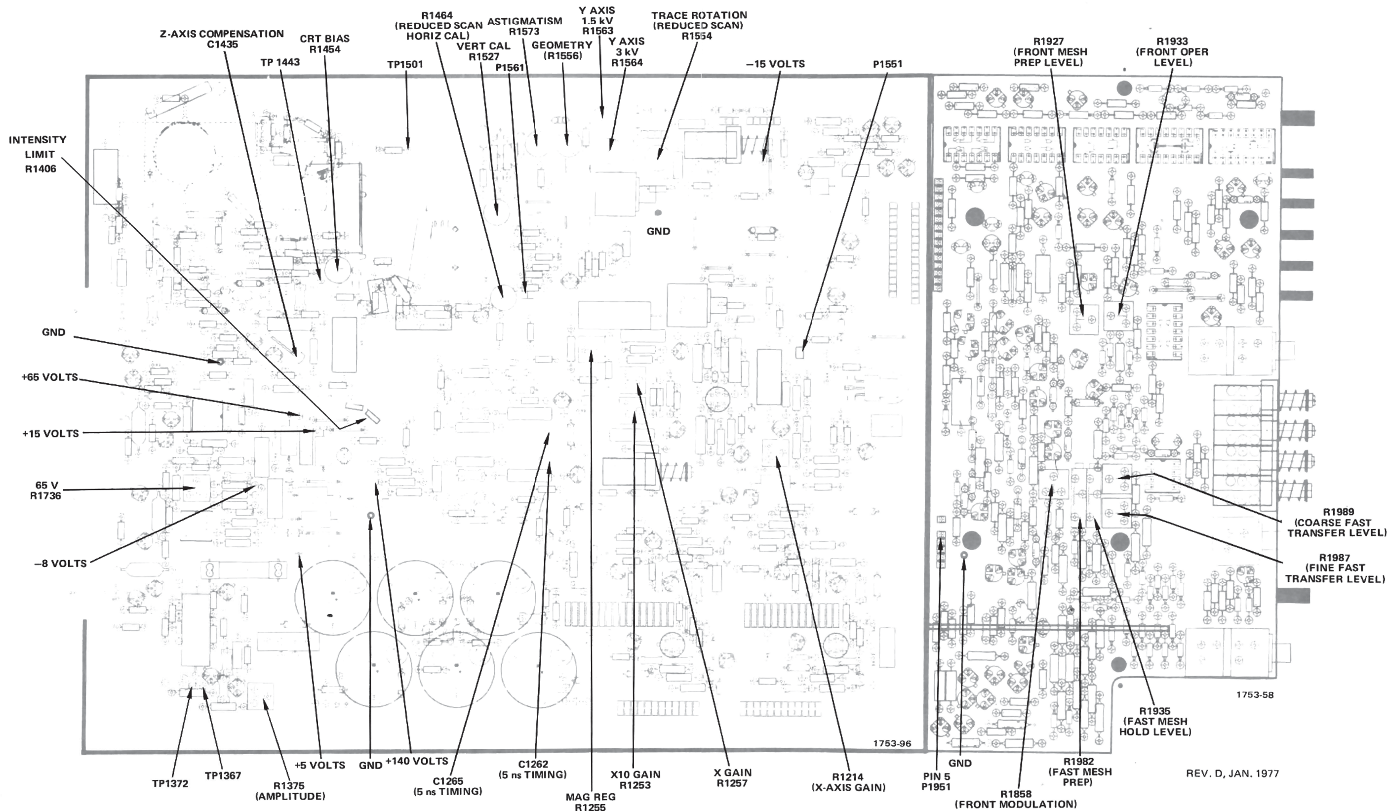
(C) Storage circuit board adjustment locations.
