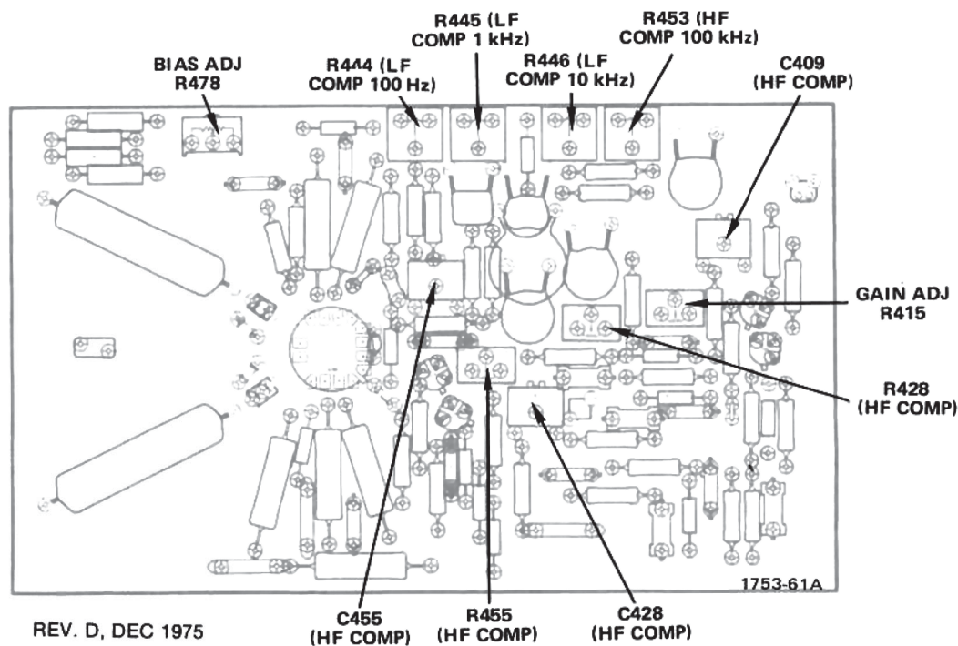
(B) Vertical Output circuit board adjustment locations.
