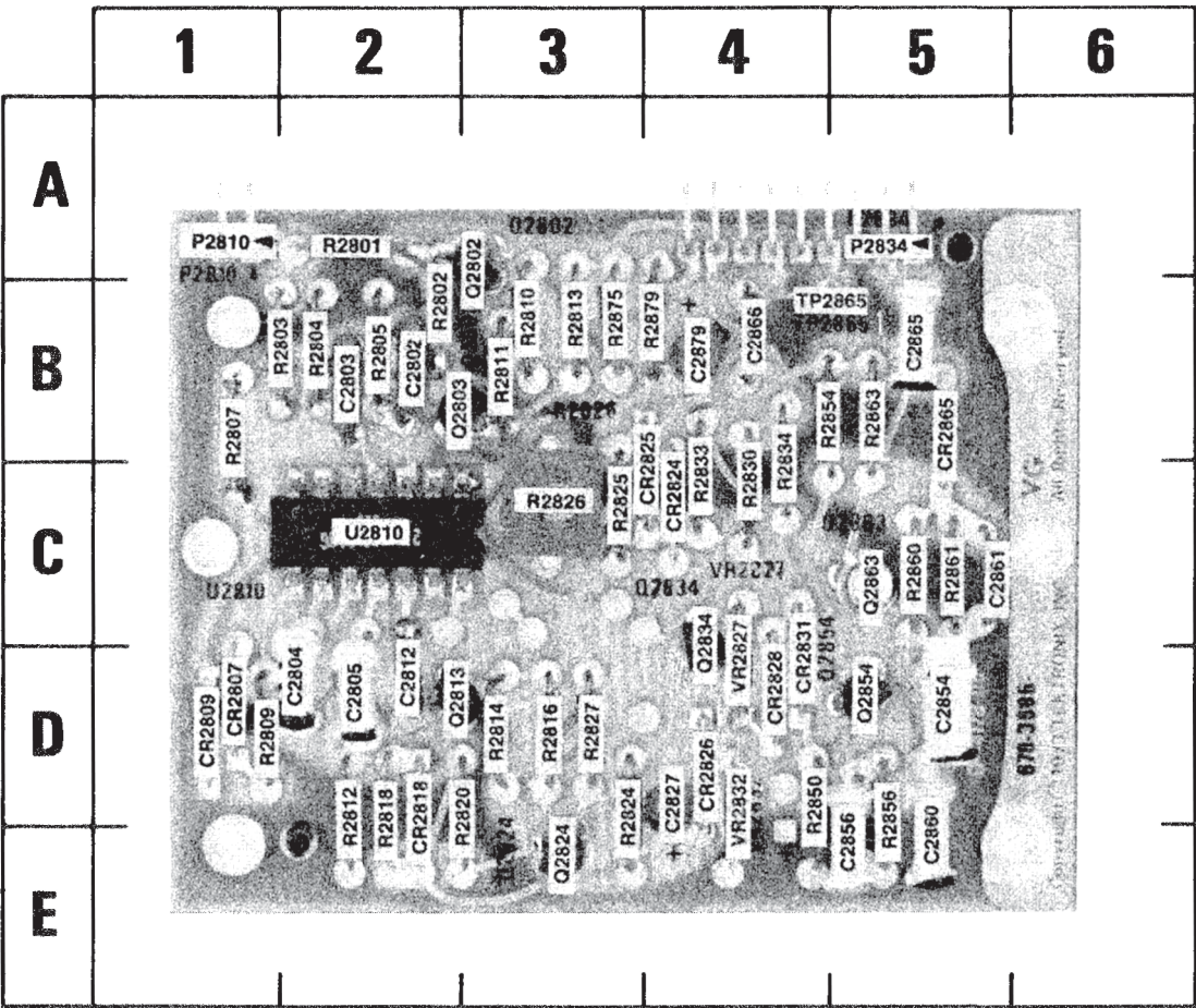
Fig. Option 5-3. A12 TV Sync Separator & Inverter Ampl board component locations.
