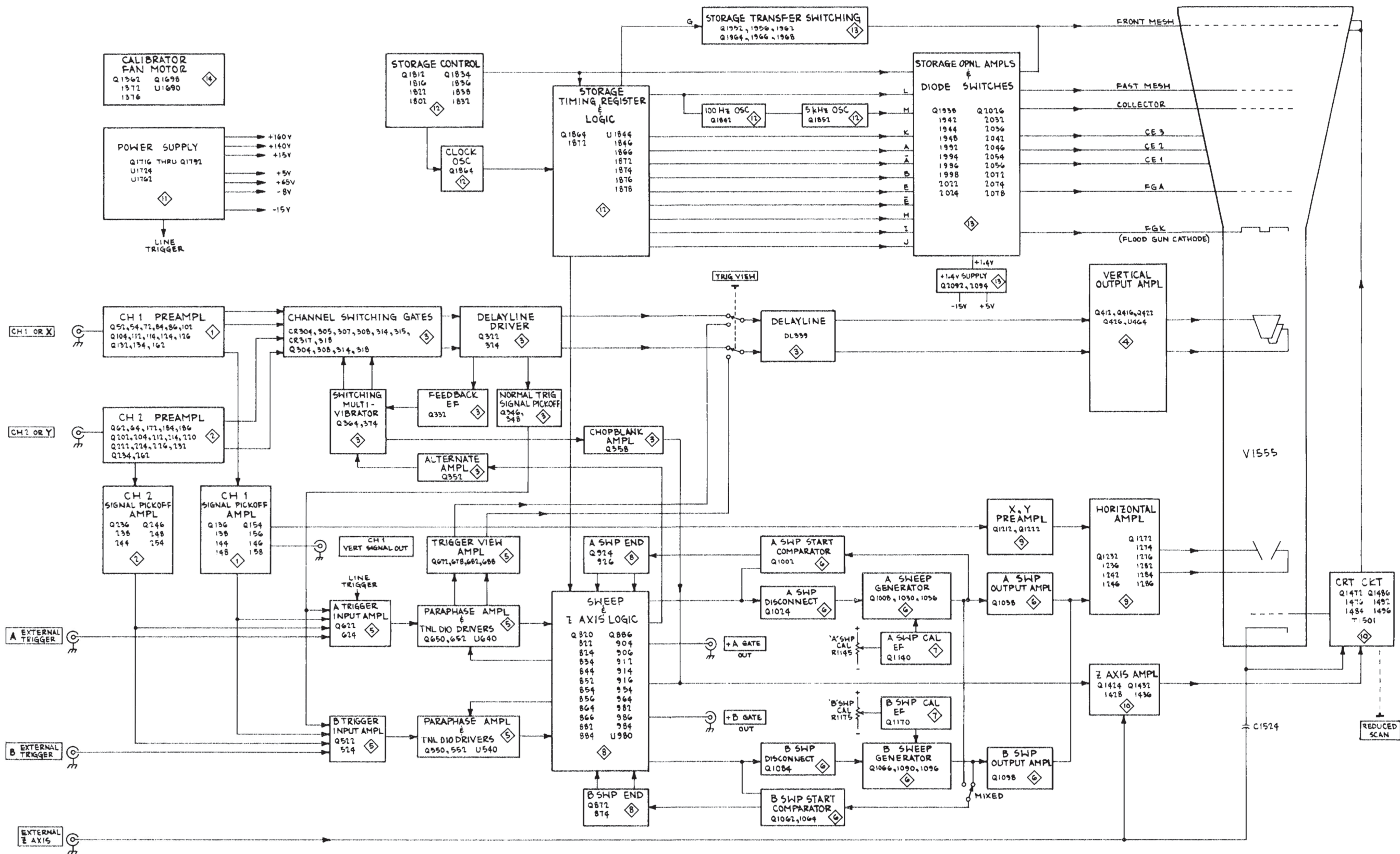
BLOCK DIAGRAM
