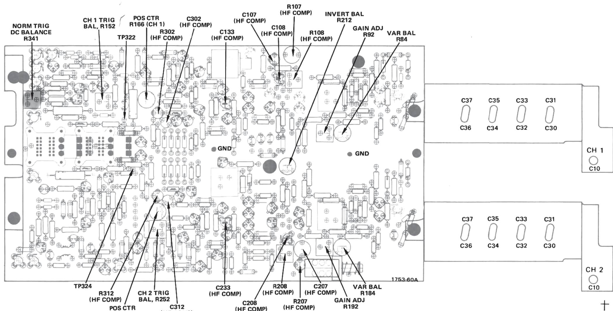
(C) Preamp circuit board adjustment locations.
