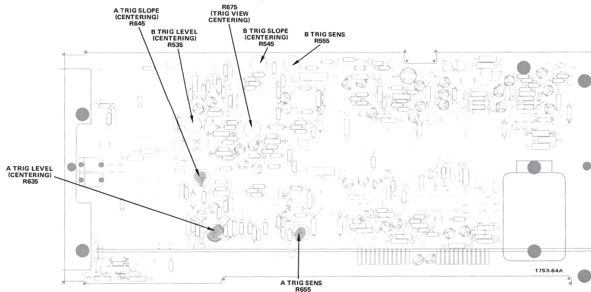
(C) Trigger circuit board adjustment locations.
