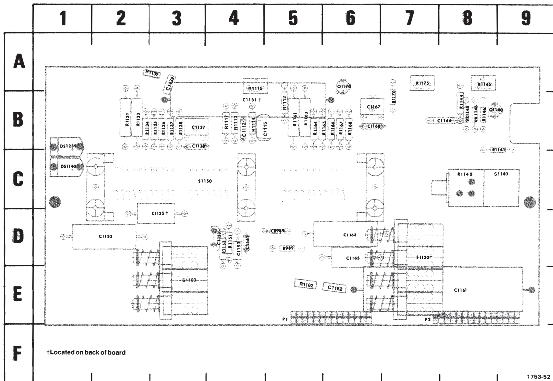
(B) A7 Timing circuit board (SN B010100-B010291)
