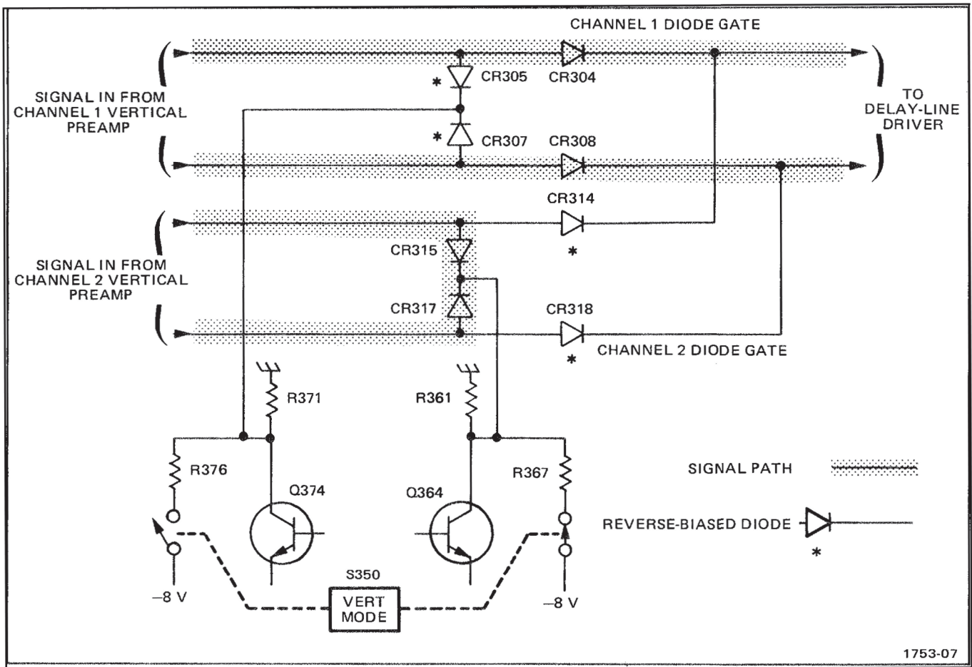
Fig. 3-4. Diode Gate Conditions in Channel 1 Mode.
