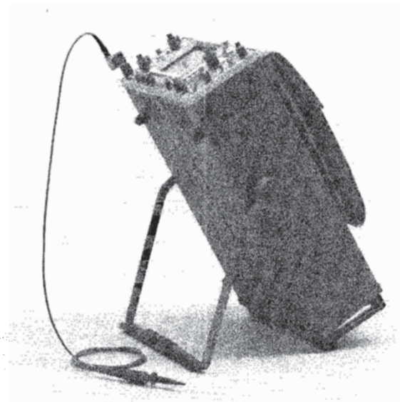
Fig. 1-1. 466 Portable Storage Oscilloscope.
