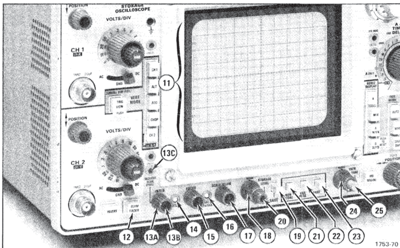
Fig. 2-3. Display and Storage Sections.
