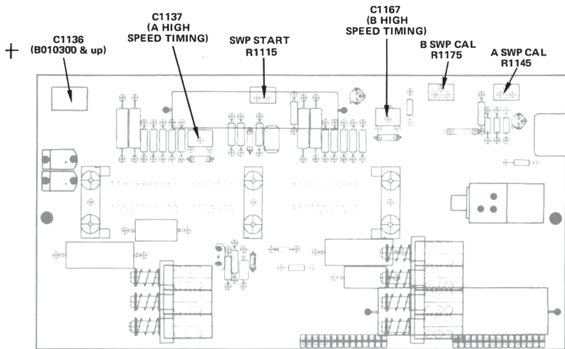
(C) Timing circuit board adjustment locations.
