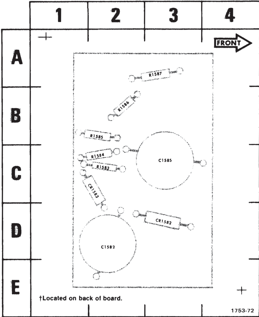
(A) A8 HV Multiplier board.
