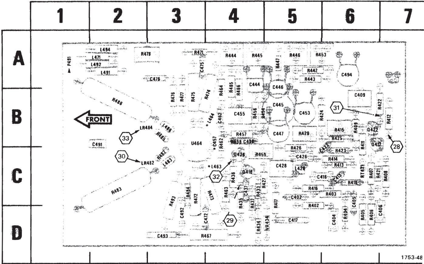
(A) A4 Vertical Output circuit board.
