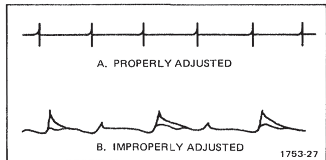
Figure Option 7-3. Inverter balance.
