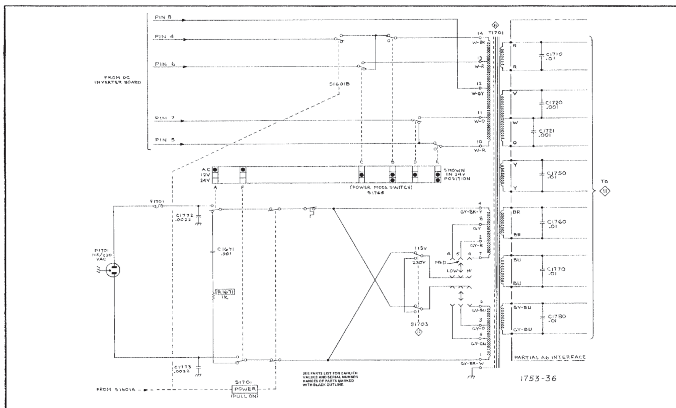
Figure Option 7-7. 466 Option 7 primary winding.
