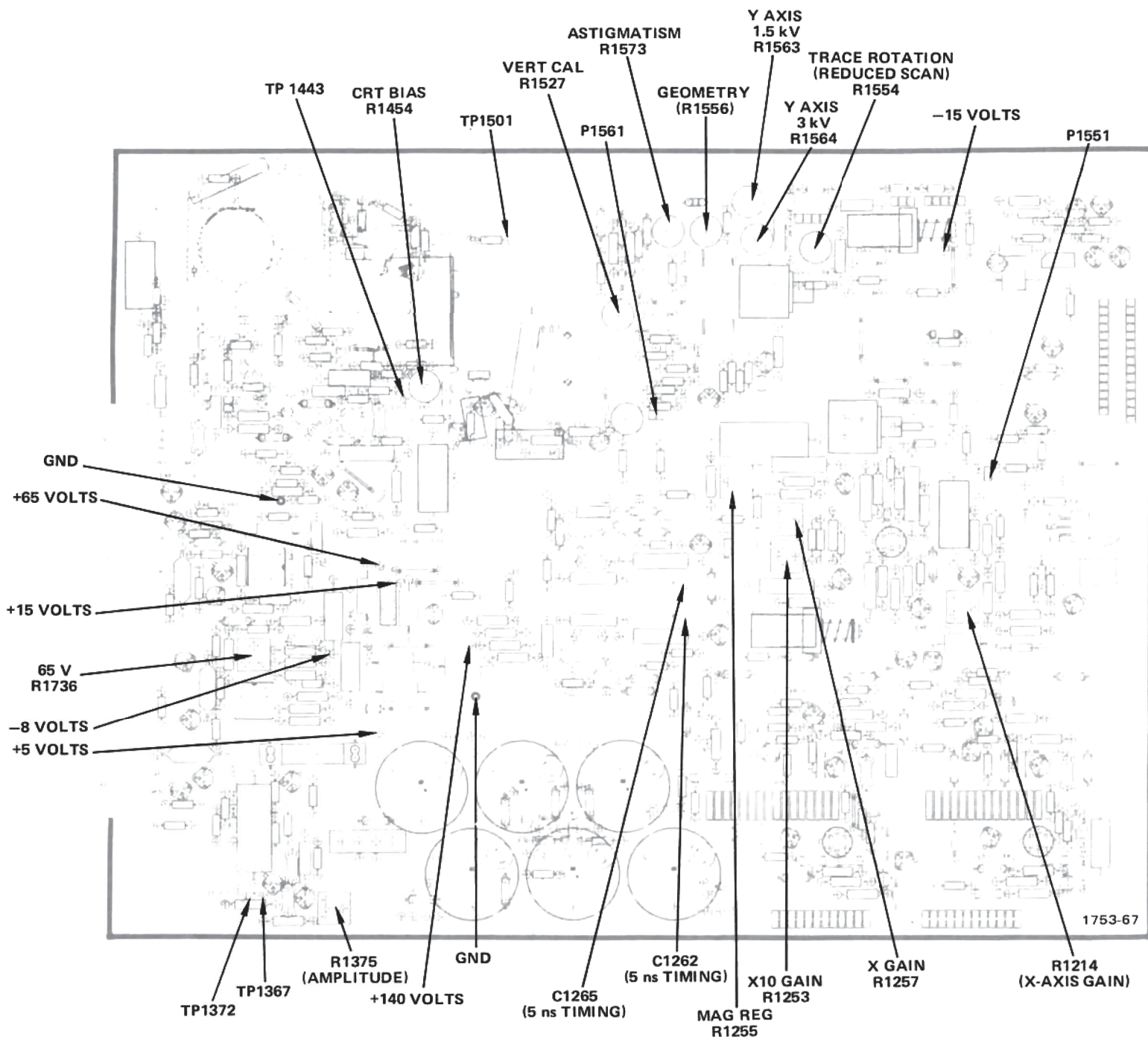
(B) Main Interface circuit board adjustment locations.
