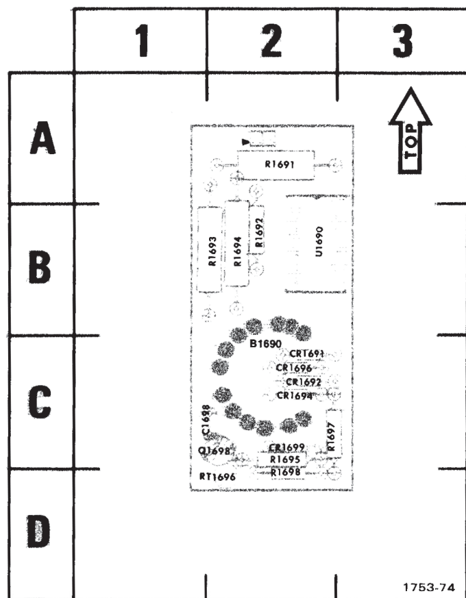
(A) A11 Fan Motor board.
