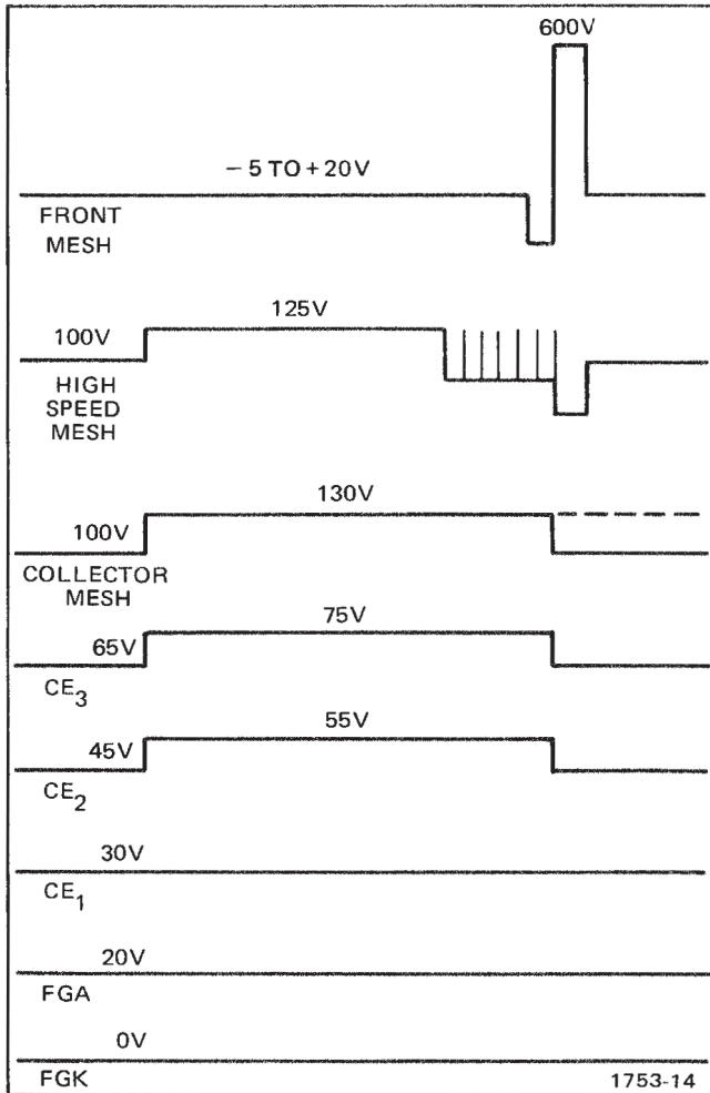
Fig. 3-14. Multi-Fast Mode—CRT Storage Element Voltage Levels.
