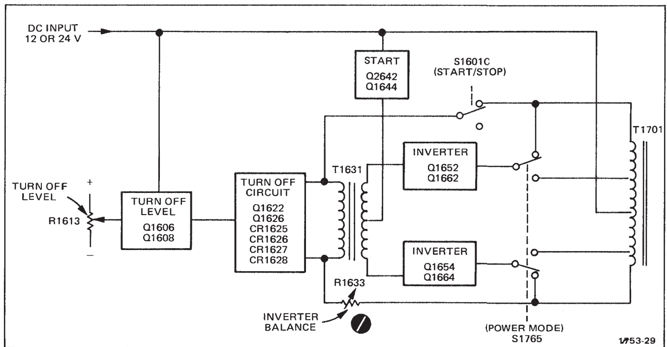
Figure Option 7-1. Option 7 simplified block diagram.
