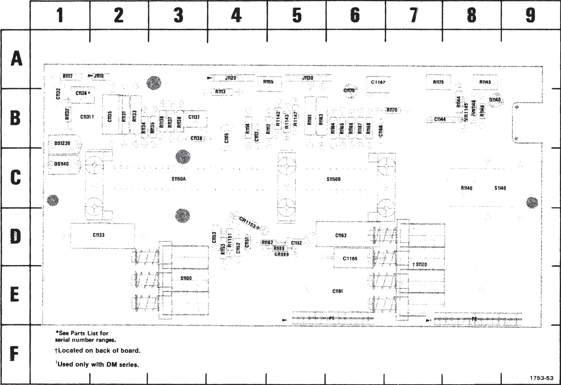
(A) A7 Timing circuit board (SN B10292-up)
