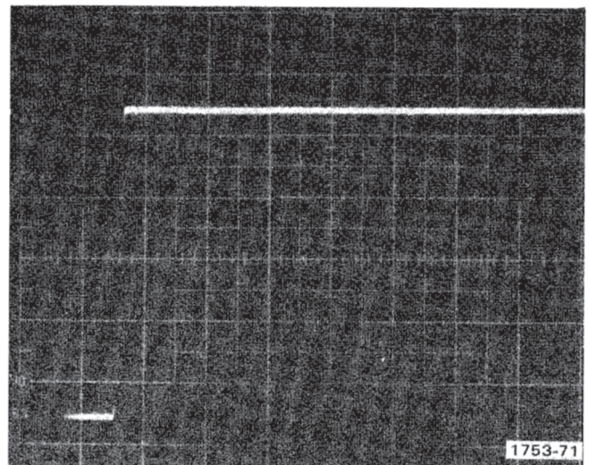
Fig. 5-C-1. Typical display when high-frequency compensation is correctly adjusted.
