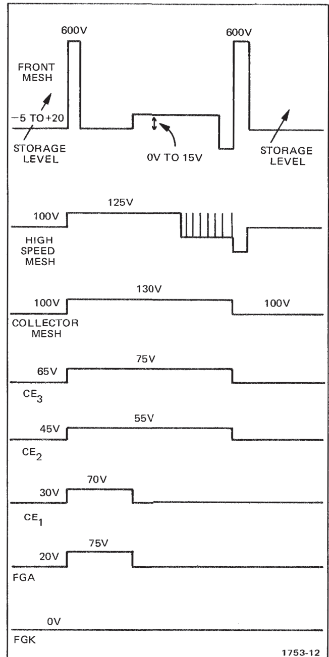
Fig. 3-13. Fast Mode—CRT Storage Element Voltage Levels.
