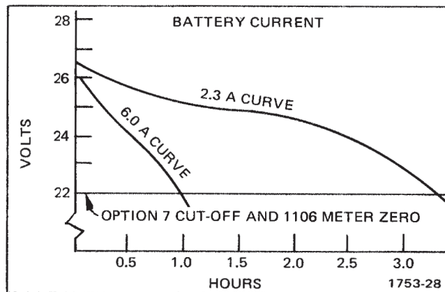
Figure Option 7-2. Typical battery pack discharge curves.
