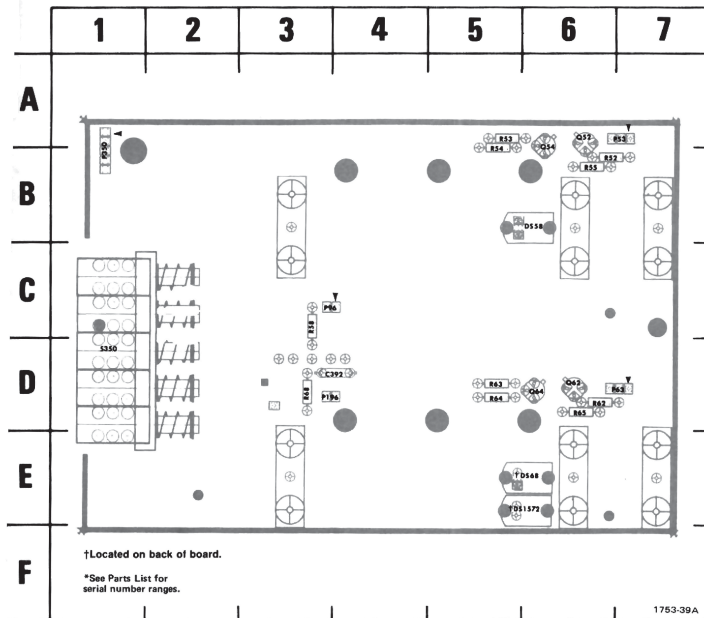
(B) A3 Vertical Mode Switch circuit board.
