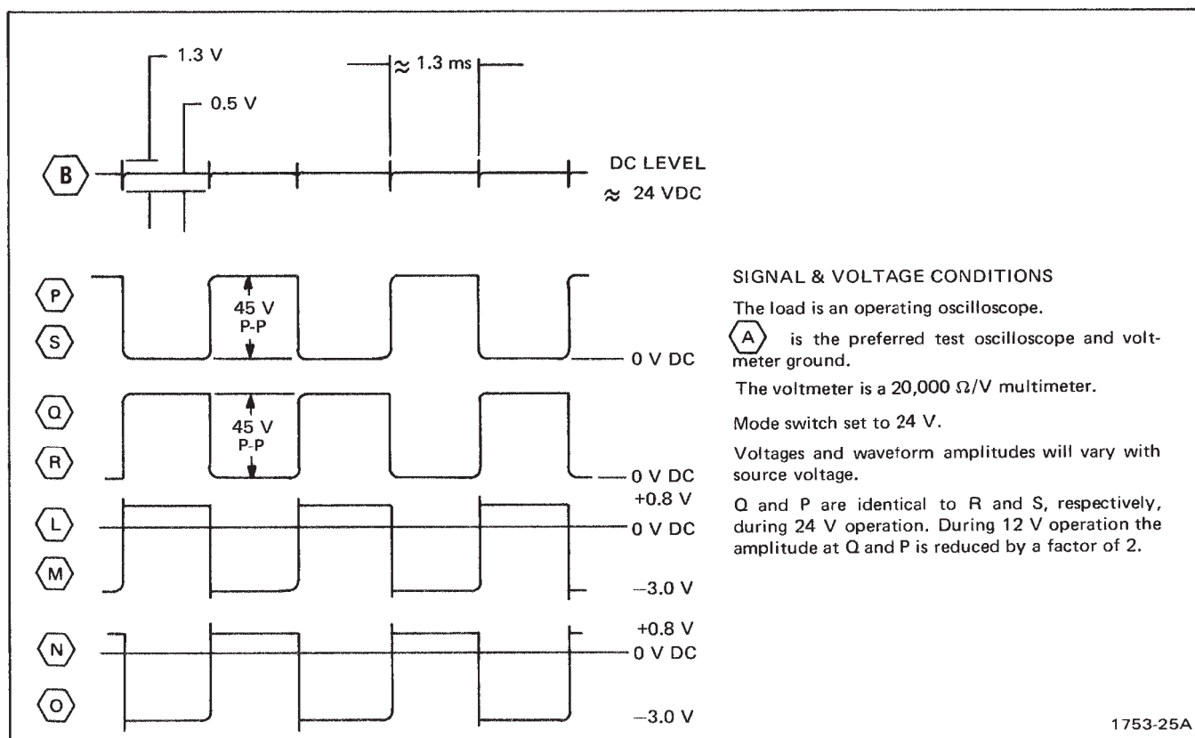
Figure Option 7-8. Typical idealized waveforms.
