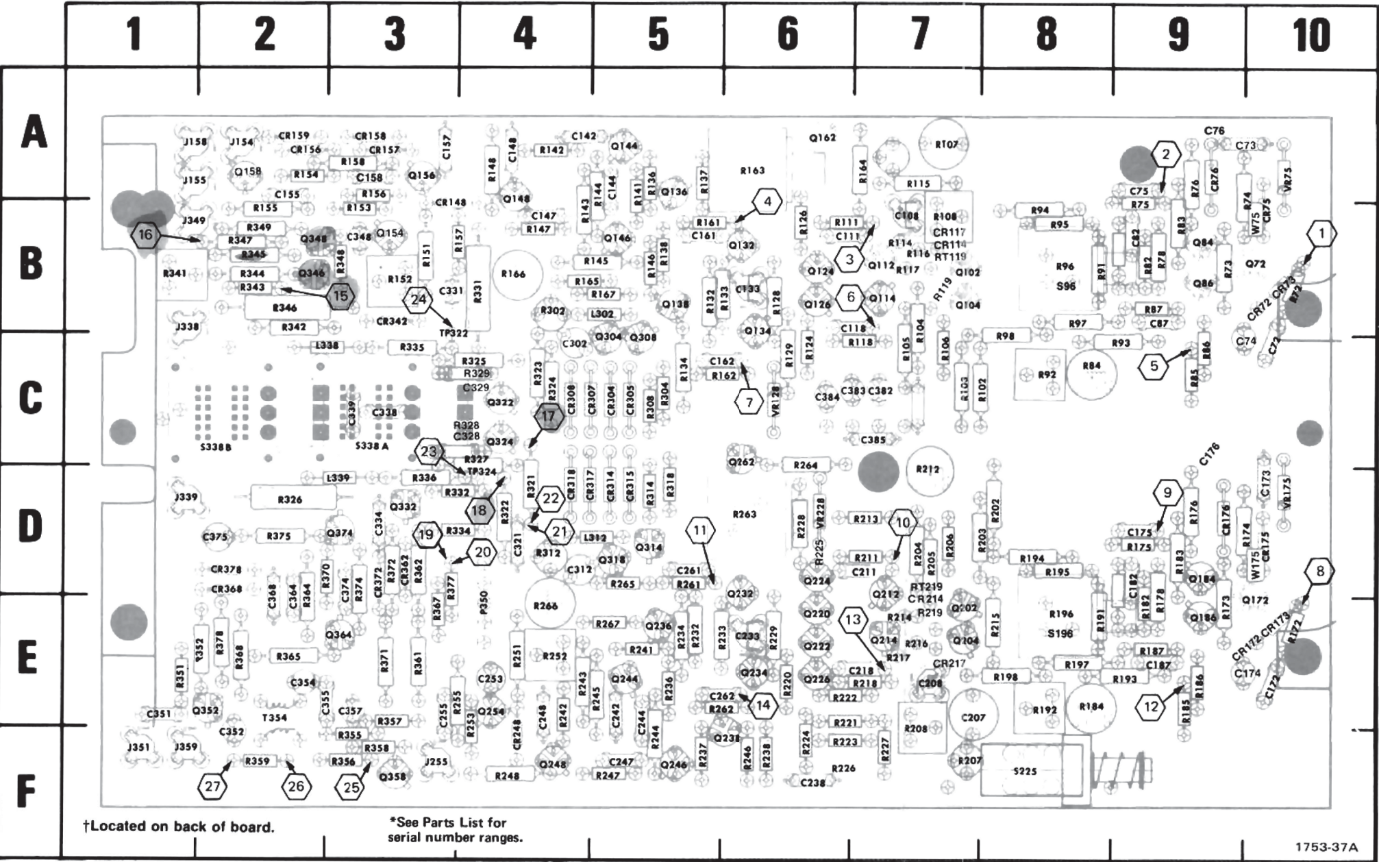
(A) A2-Vertical Preamp circuit board.
