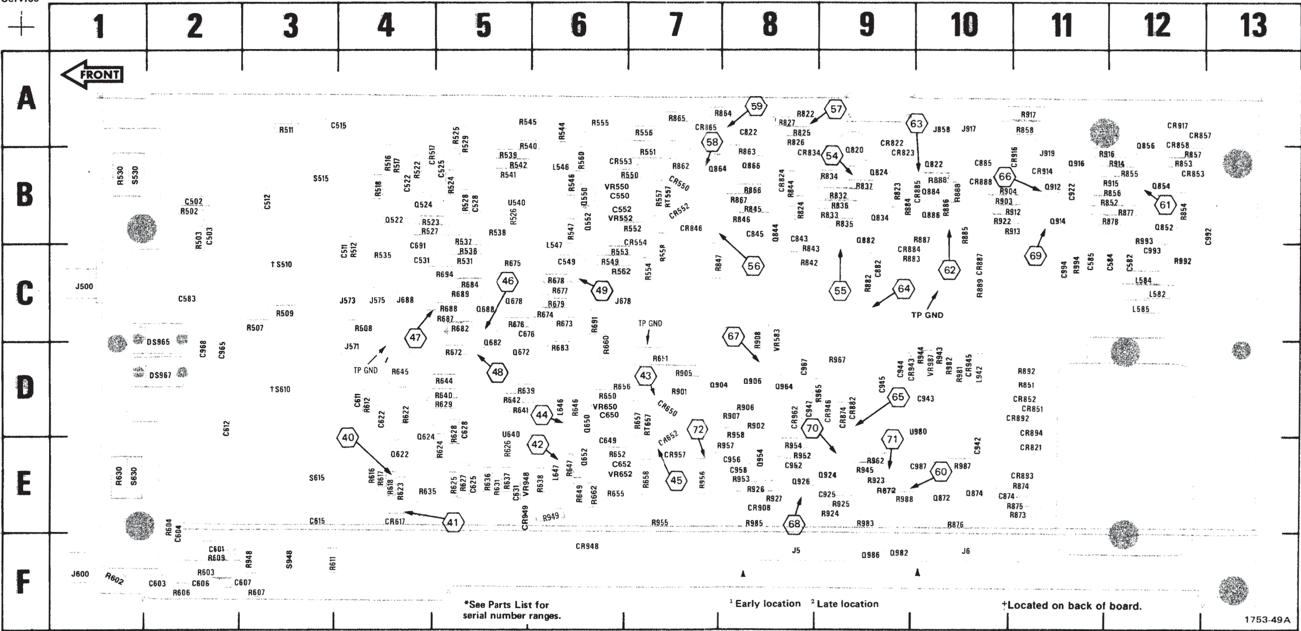
(A) A5 Trigger Generator and Sweep Logic circuit board.
